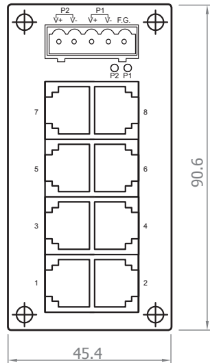
Front-panel view
